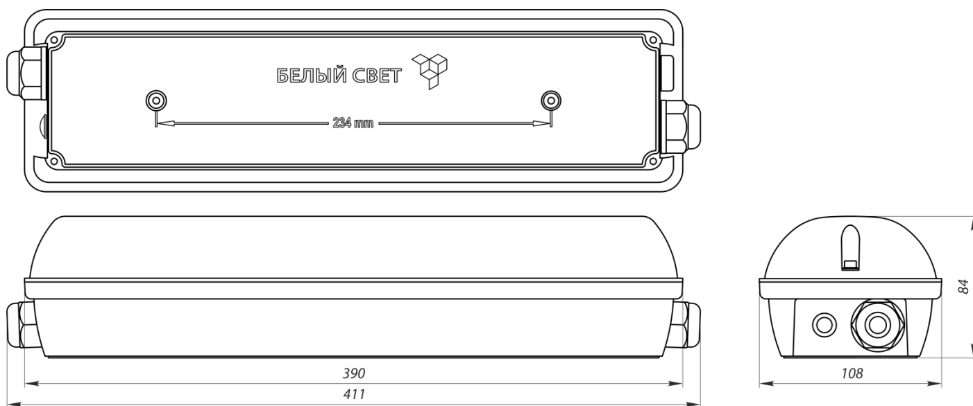
Рис. 6 БАП BS-STABILAR2-81-B2-UNI BOX IP66 (1,0-45 W / = 190-260 V)
